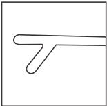
1M-10-605 LESTER Lens Pusher Shaft with 0.25 mm Dia Hour-Glass Shape Tip
